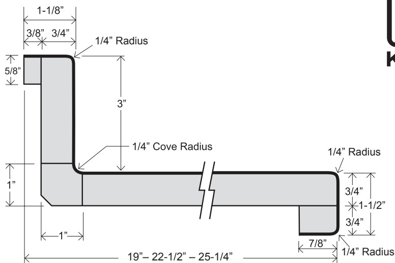
KITCHEN & VANITY TOP CNV 19 CNV 22-1/2 CNK 25-1/4
